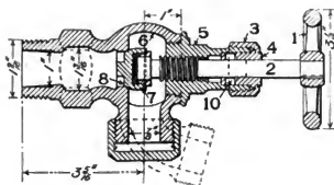
Fig. 3017. 3/4-Inch Angle Valve.
